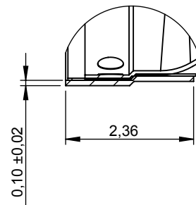
DETAIL B SCALE 2 : 5
